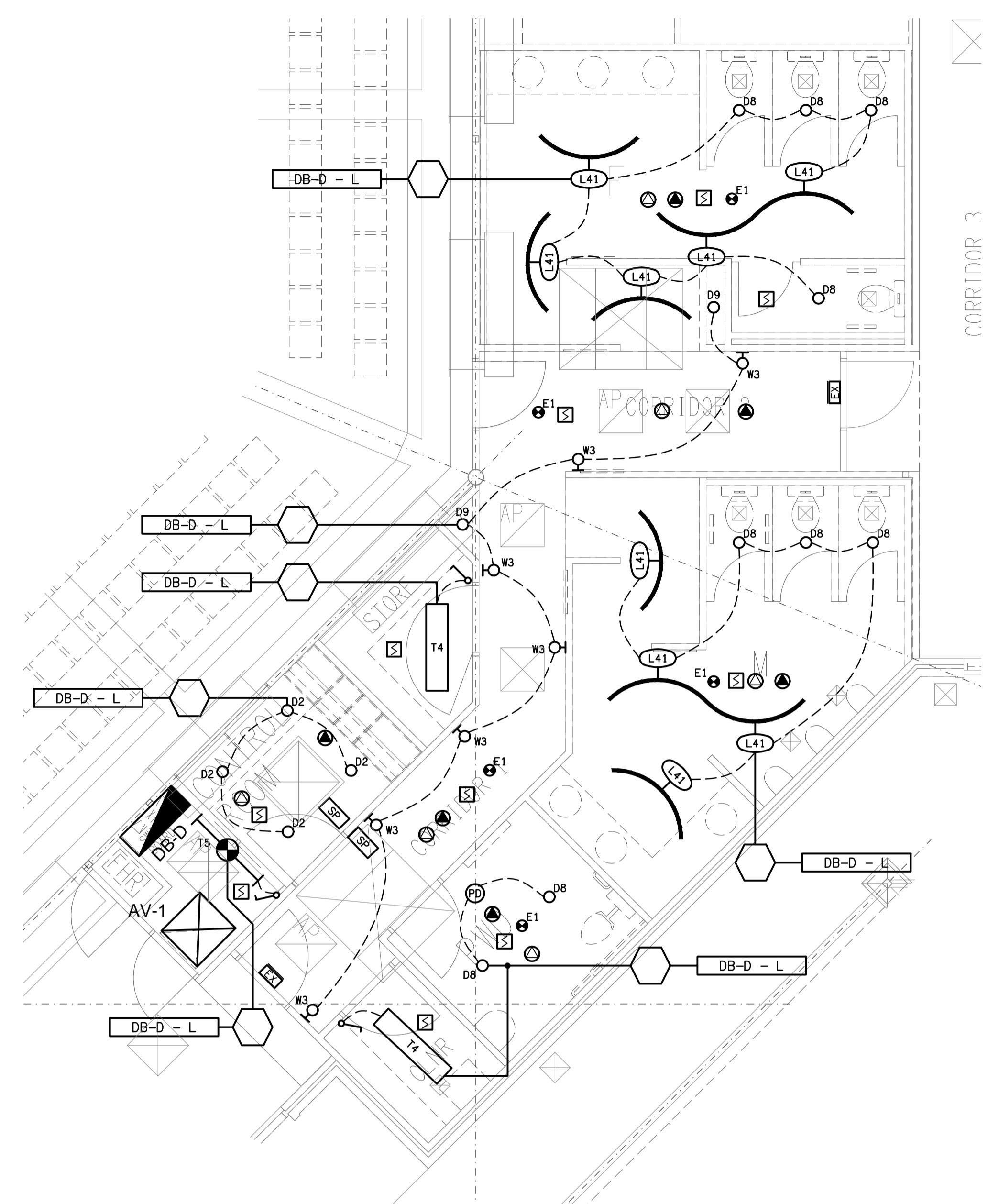
DETAIL A AMENITIES REFLECTED CEILING PLAN SCALE 1: 50
